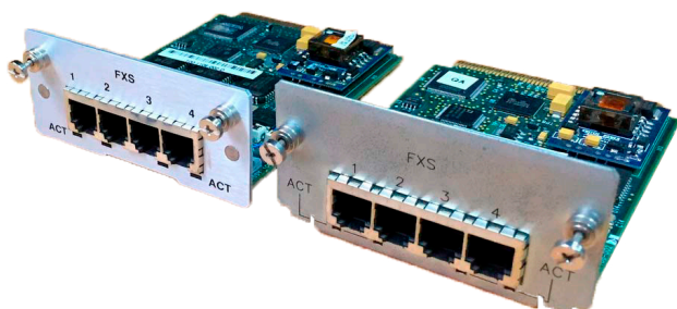
Figure 2: Low profile and regular interface cards
